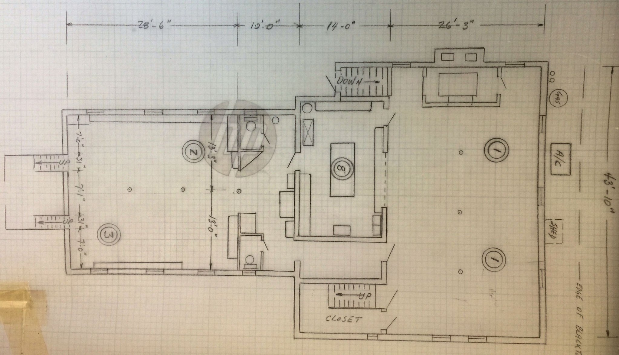
Indian Head UMC Floor Plan | Lower Level
