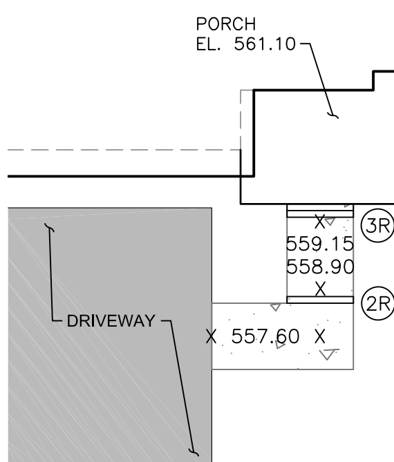
FRONT WALK DETAIL SCALE: 1" = 10'
